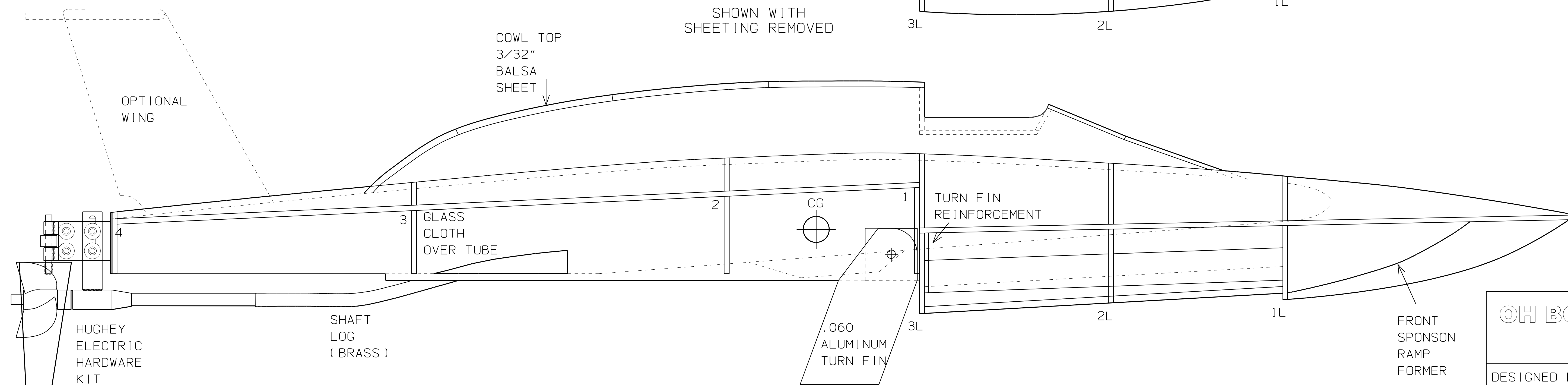
SIDE VIEW SHOWN WITH SHEETING REMOVED
